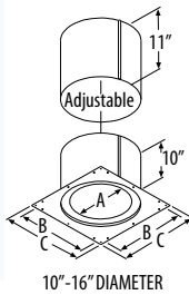
10"-16" DIAMETER
