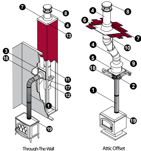
Through-The-Wall
