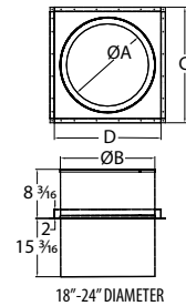
18"-24" DIAMETER
