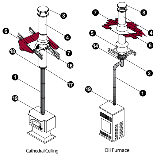
Cathedral Ceiling
